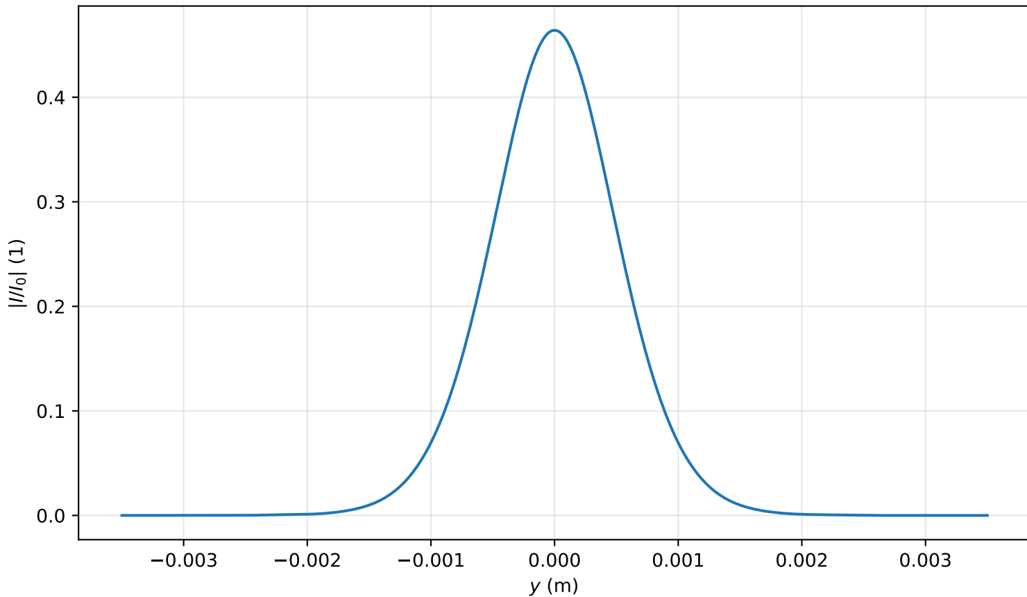
Intensity profile I(x = 0, y, z = 3.105)/I_0 , P_{in}=0.4P_{cr} , artificial time
